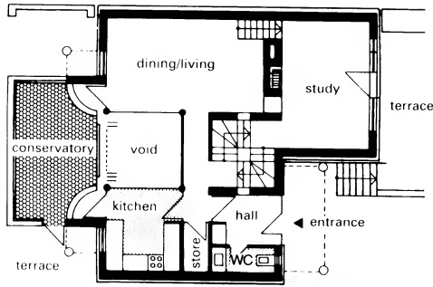
1 Ground floor → 2 + 3
